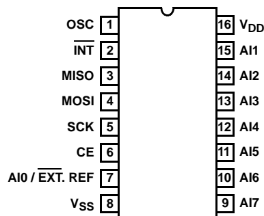
CDP68HC68A2E (PDIP) TOP VIEW
