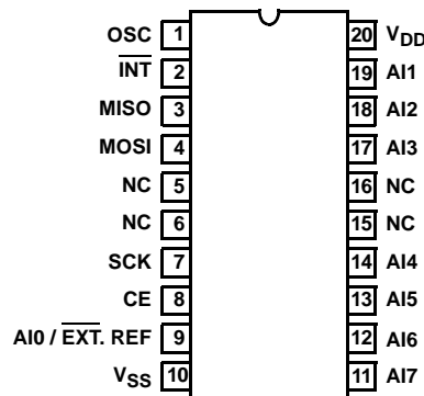
CDP68HC68A2M (SOIC) TOP VIEW
